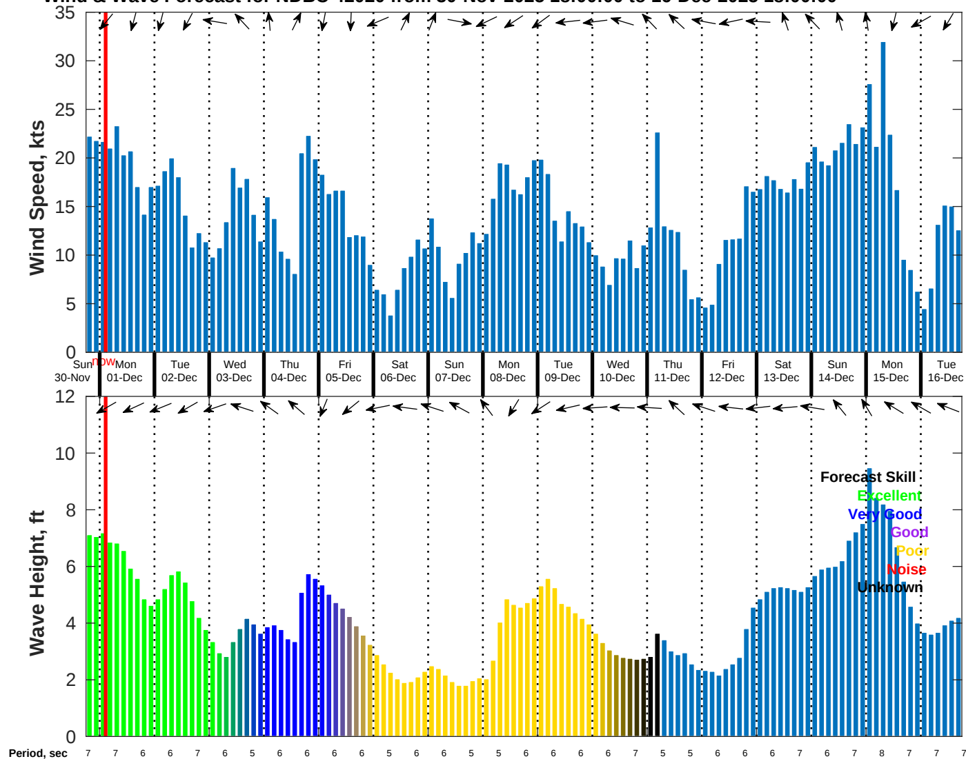
Wind & Wave Forecast for NDBC 42020 from 30-Nov-2025 18:00:00 to 16-Dec-2025 18:00:00
