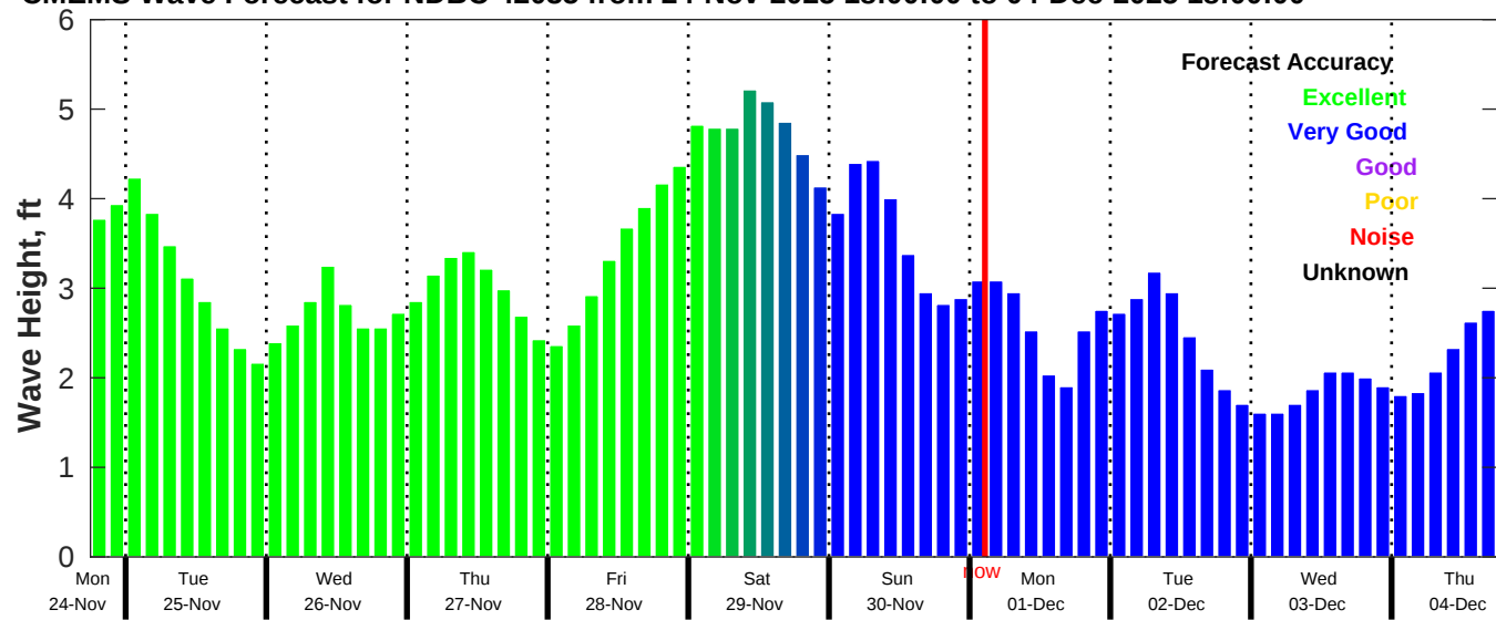
CMEMS Wave Forecast for NDBC 42035 from 24-Nov-2025 18:00:00 to 04-Dec-2025 18:00:00
