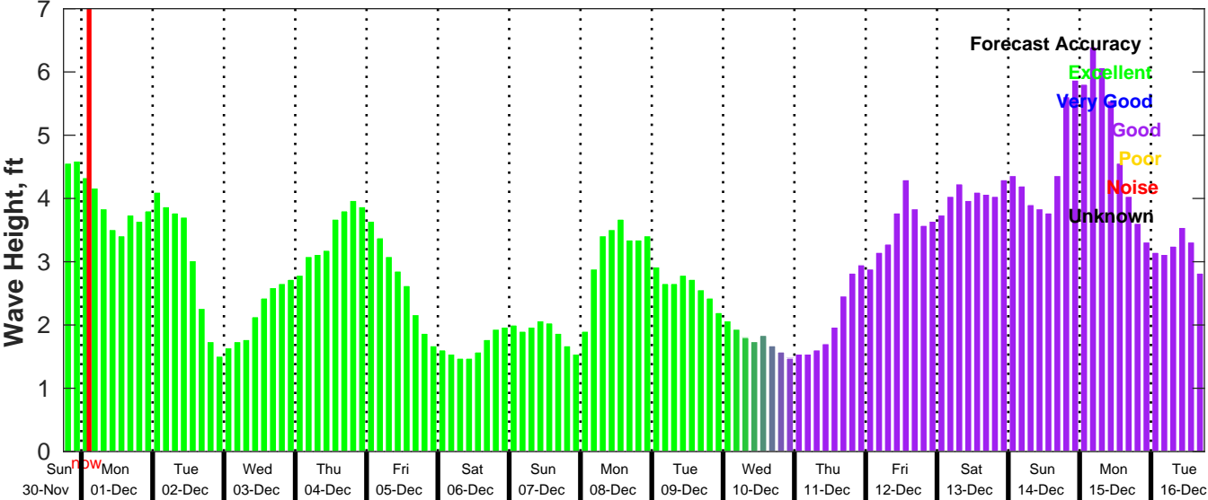
GFS Wave Forecast for NDBC 42035 from 30-Nov-2025 18:00:00 to 16-Dec-2025 18:00:00
