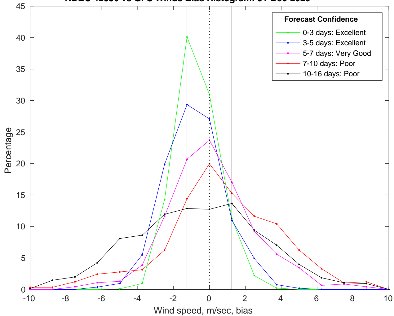
NDBC 42036 vs GFS Winds Bias Histogram: 01-Dec-2025
