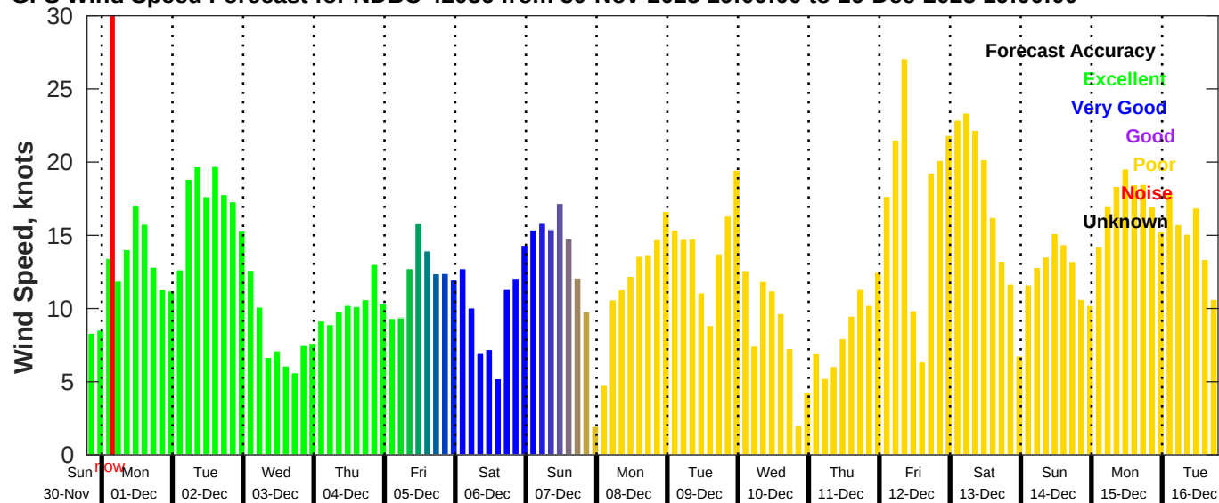
GFS Wind Speed Forecast for NDBC 42036 from 30-Nov-2025 19:00:00 to 16-Dec-2025 19:00:00
