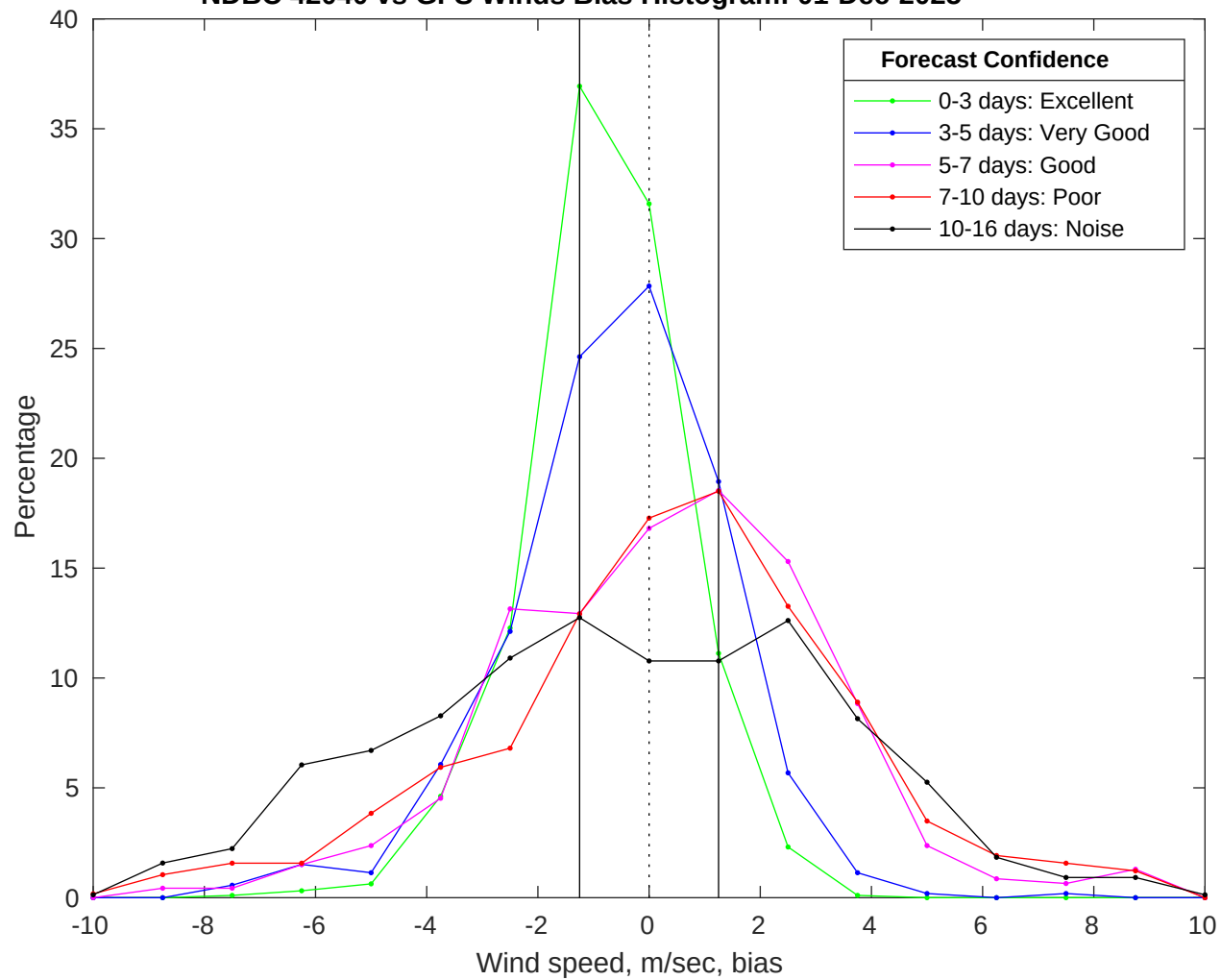
NDBC 42040 vs GFS Winds Bias Histogram: 01-Dec-2025
