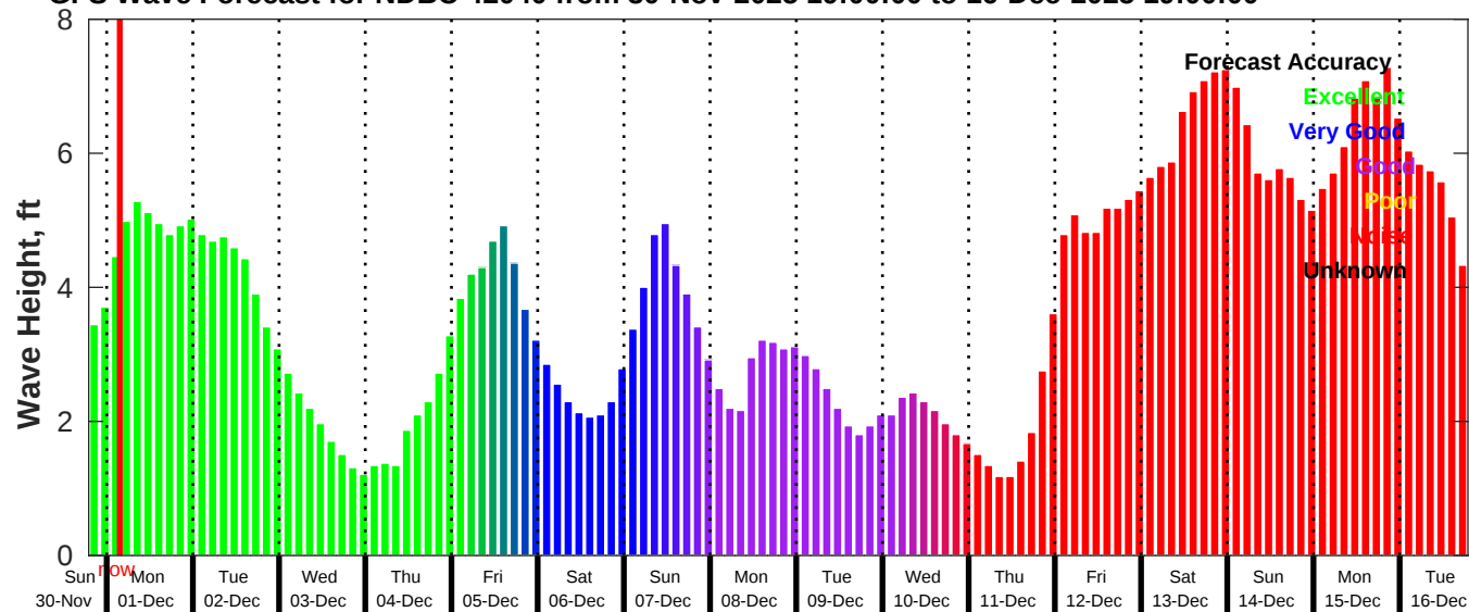
GFS Wave Forecast for NDBC 42040 from 30-Nov-2025 19:00:00 to 16-Dec-2025 19:00:00
