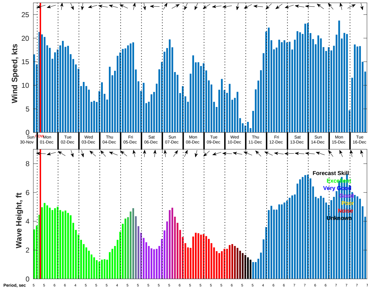
Wind & Wave Forecast for NDBC 42040 from 30-Nov-2025 19:00:00 to 16-Dec-2025 19:00:00
