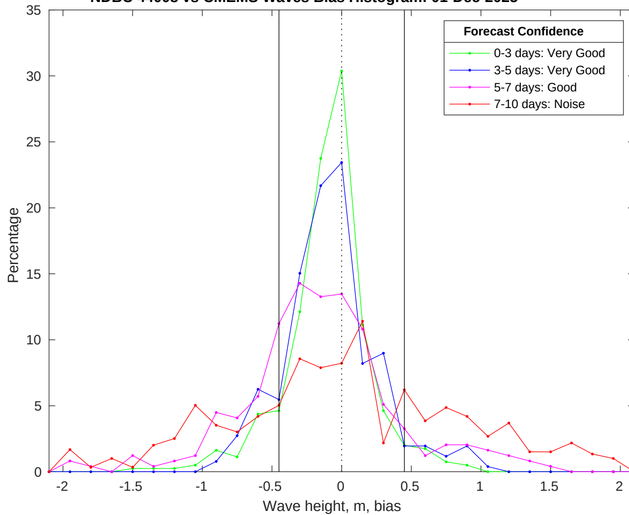
NDBC 44008 vs CMEMS Waves Bias Histogram: 01-Dec-2025
