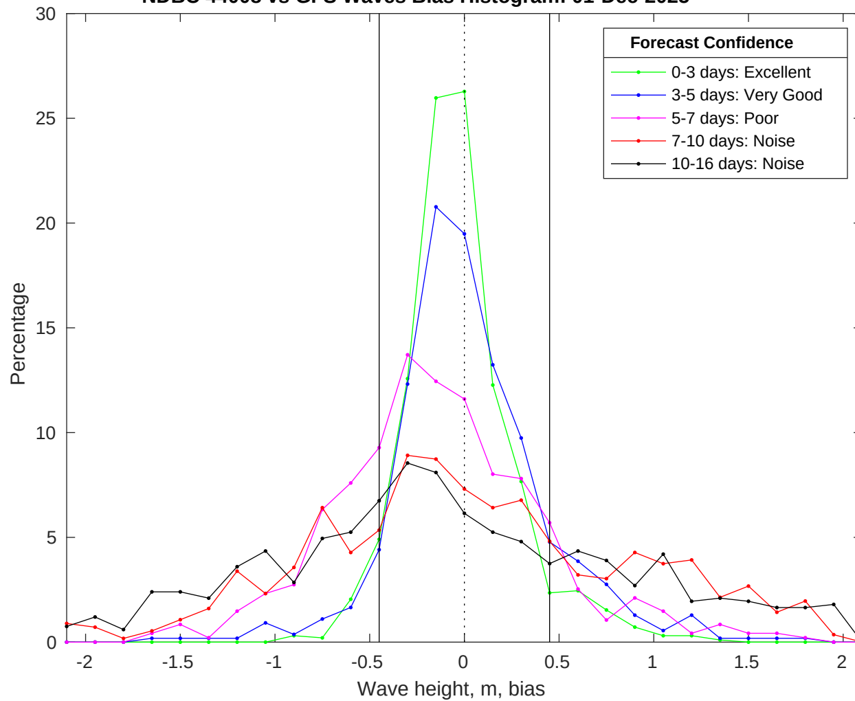
NDBC 44008 vs GFS Waves Bias Histogram: 01-Dec-2025
