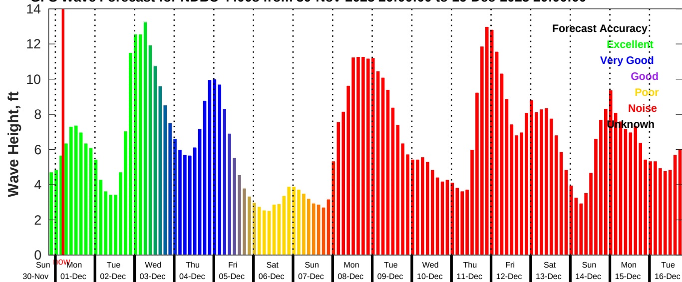
GFS Wave Forecast for NDBC 44008 from 30-Nov-2025 20:00:00 to 16-Dec-2025 20:00:00
