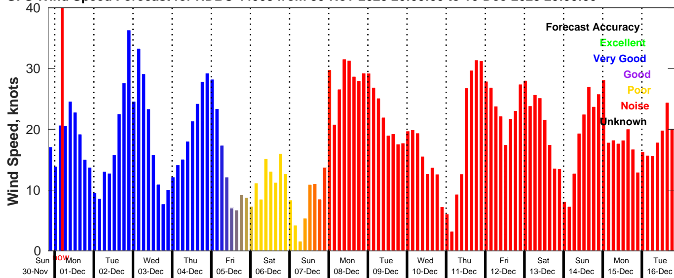
GFS Wind Speed Forecast for NDBC 44008 from 30-Nov-2025 20:00:00 to 16-Dec-2025 20:00:00
