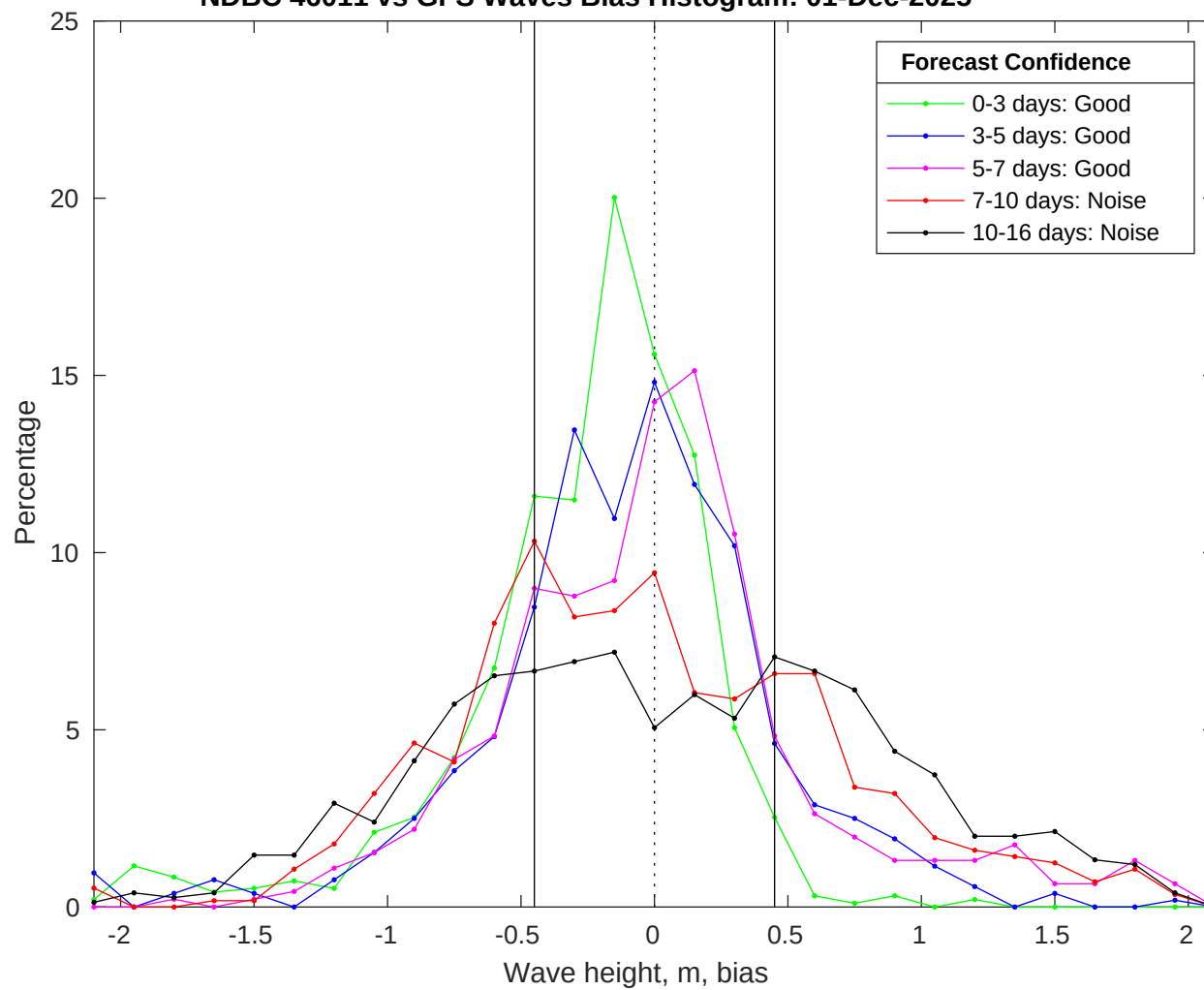
NDBC 46011 vs GFS Waves Bias Histogram: 01-Dec-2025
