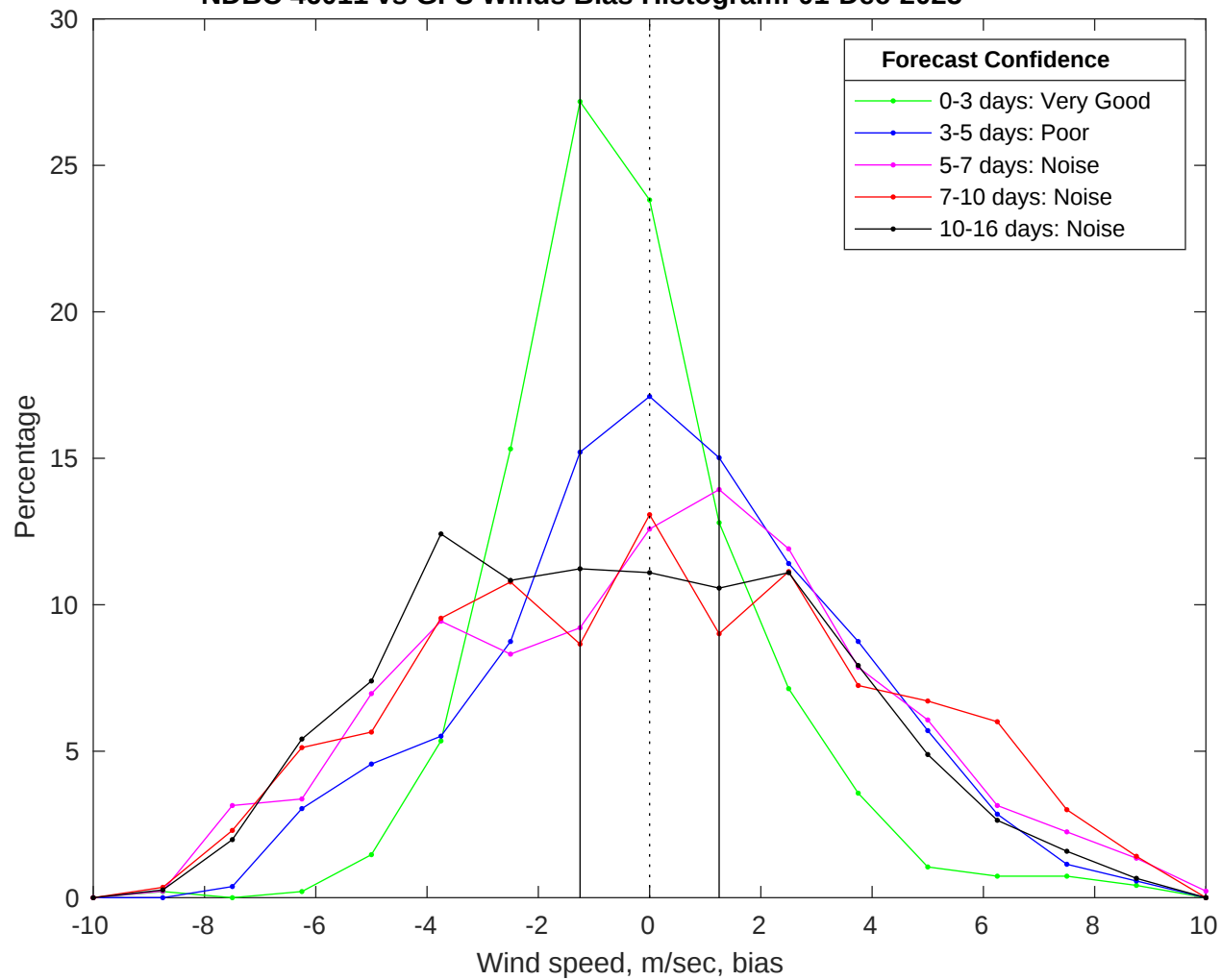
NDBC 46011 vs GFS Winds Bias Histogram: 01-Dec-2025
