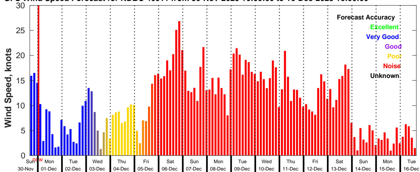
GFS Wind Speed Forecast for NDBC 46011 from 30-Nov-2025 16:00:00 to 16-Dec-2025 16:00:00
