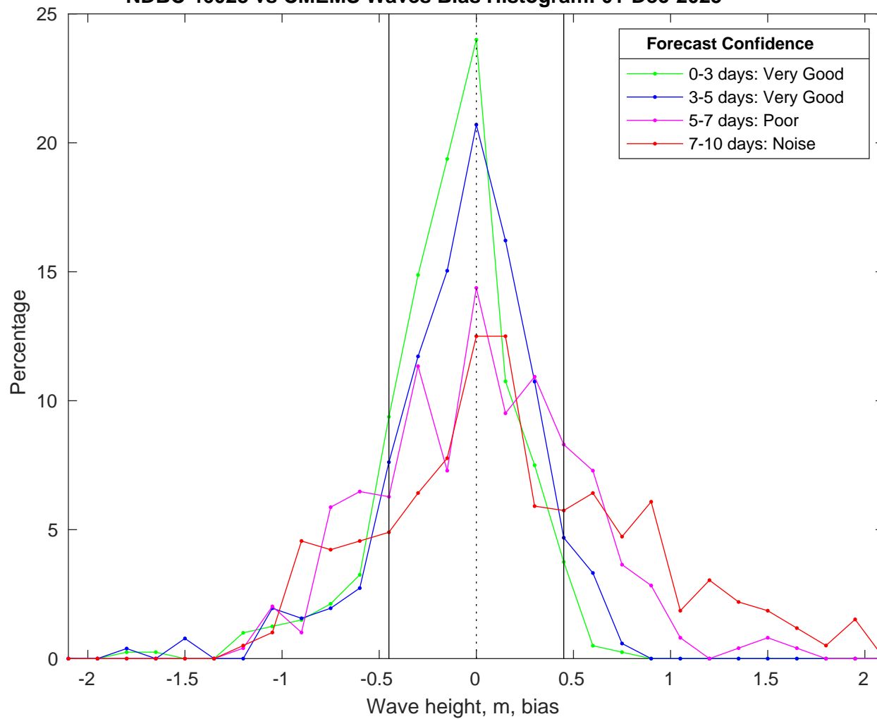
NDBC 46028 vs CMEMS Waves Bias Histogram: 01-Dec-2025
