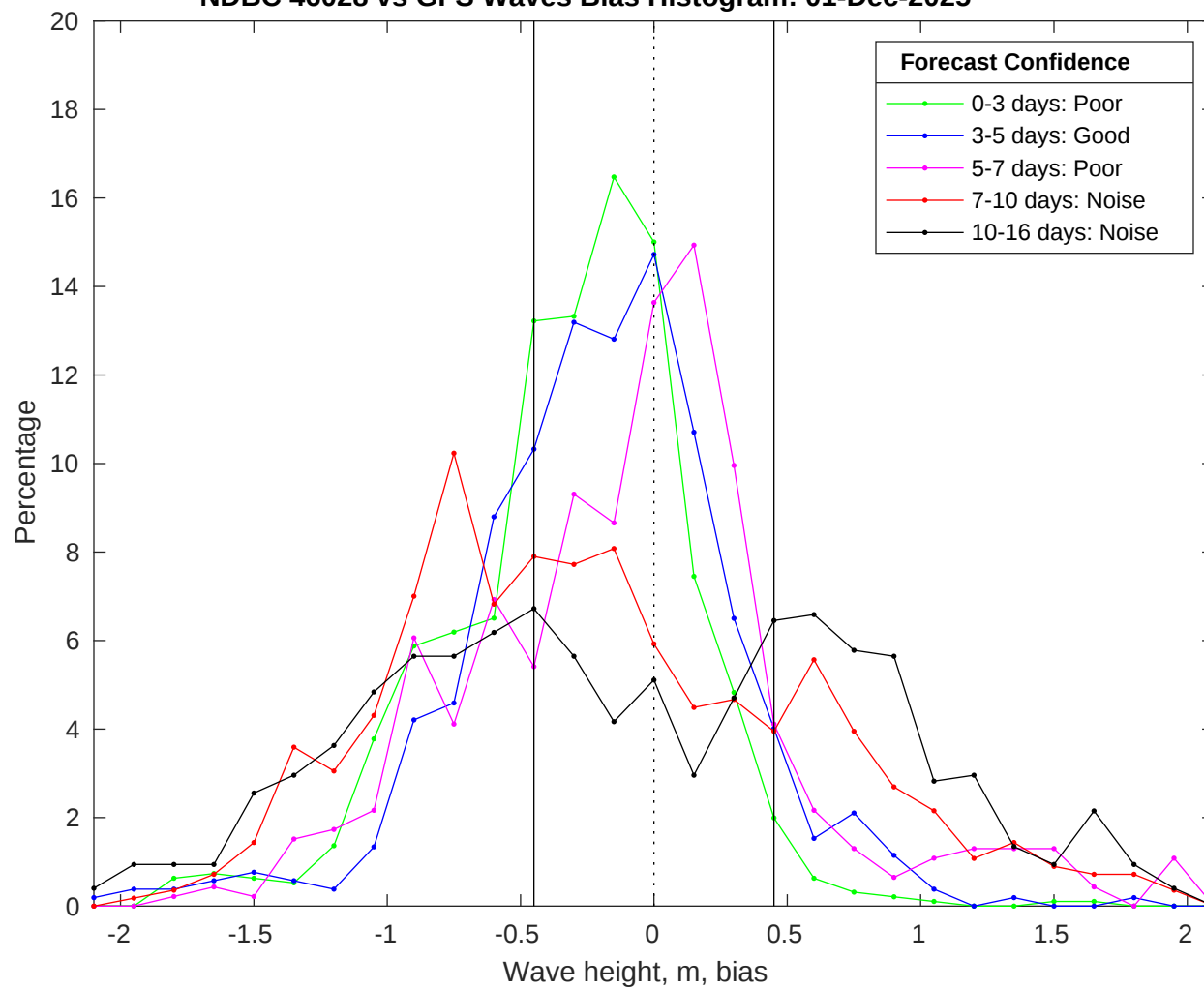
NDBC 46028 vs GFS Waves Bias Histogram: 01-Dec-2025
