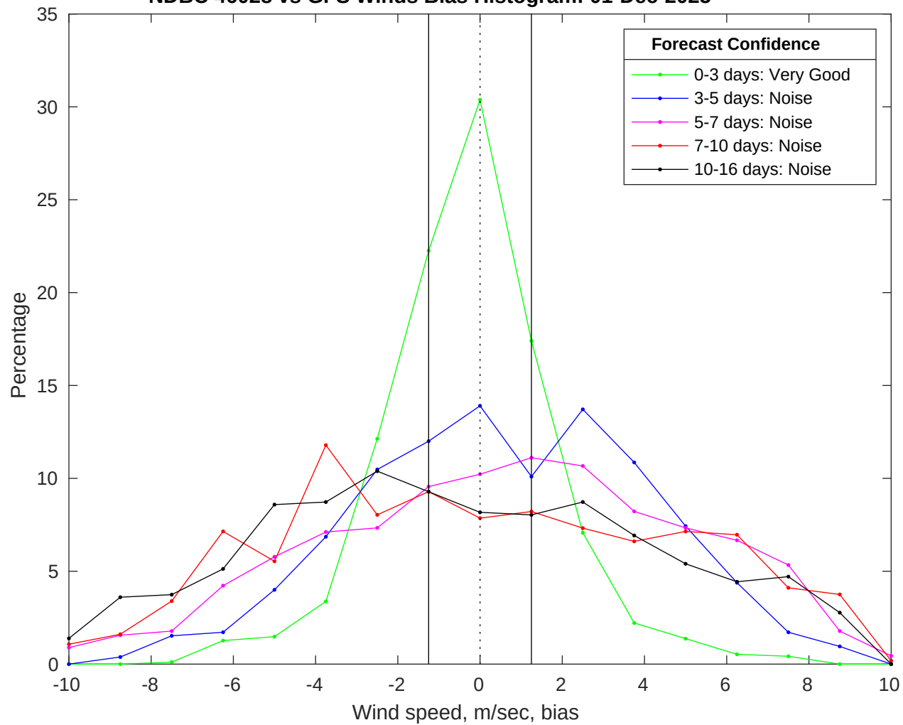
NDBC 46028 vs GFS Winds Bias Histogram: 01-Dec-2025
