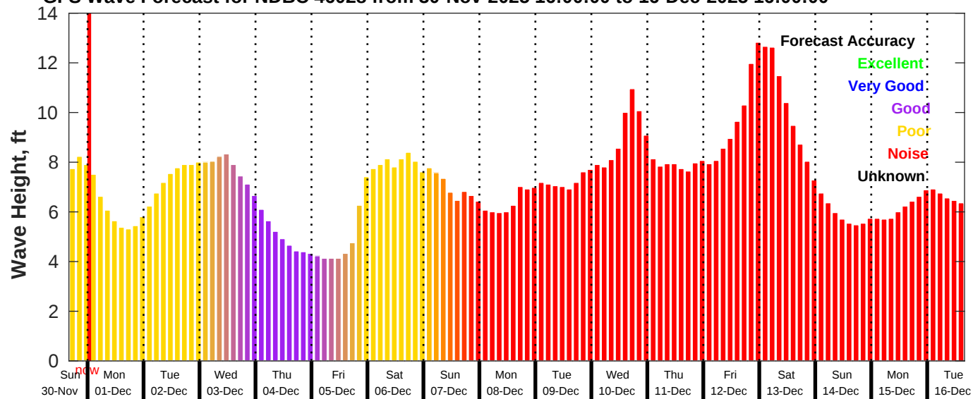
GFS Wave Forecast for NDBC 46028 from 30-Nov-2025 16:00:00 to 16-Dec-2025 16:00:00
