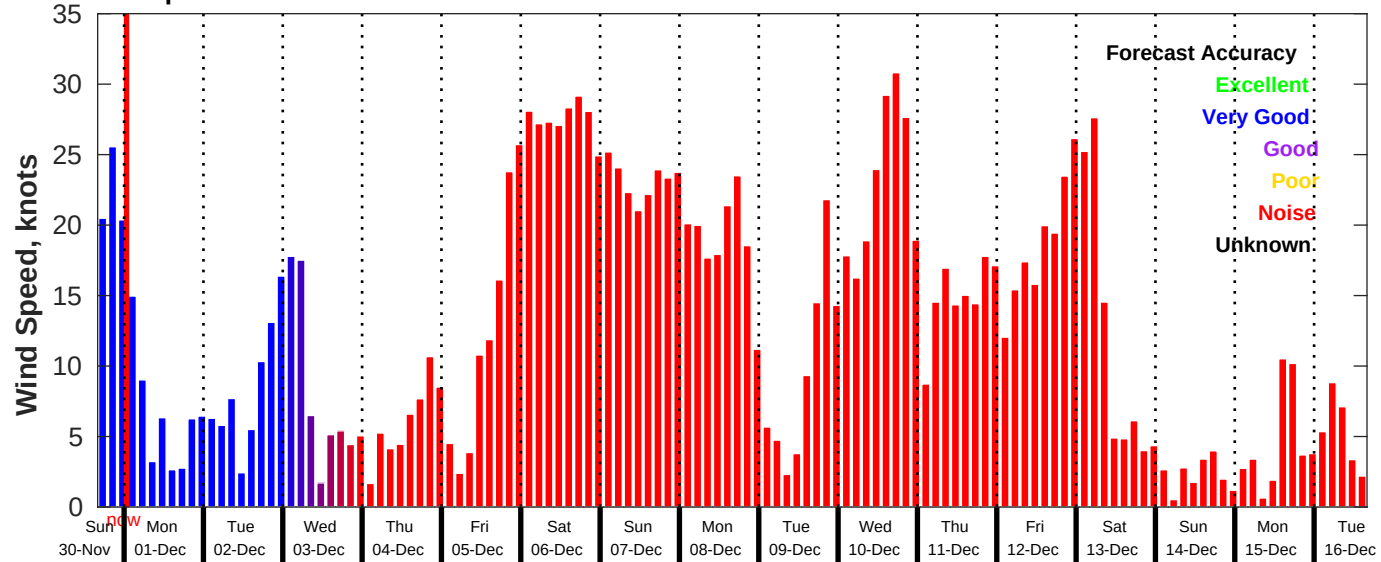
GFS Wind Speed Forecast for NDBC 46028 from 30-Nov-2025 16:00:00 to 16-Dec-2025 16:00:00
