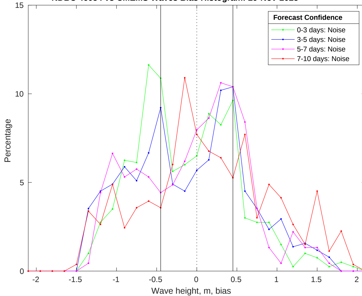
NDBC 46054 vs CMEMS Waves Bias Histogram: 29-Nov-2025
