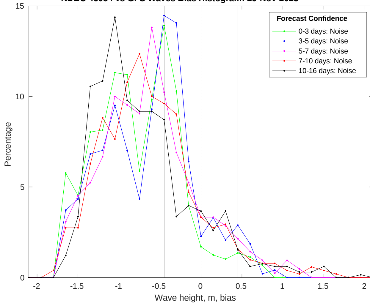
NDBC 46054 vs GFS Waves Bias Histogram: 29-Nov-2025
