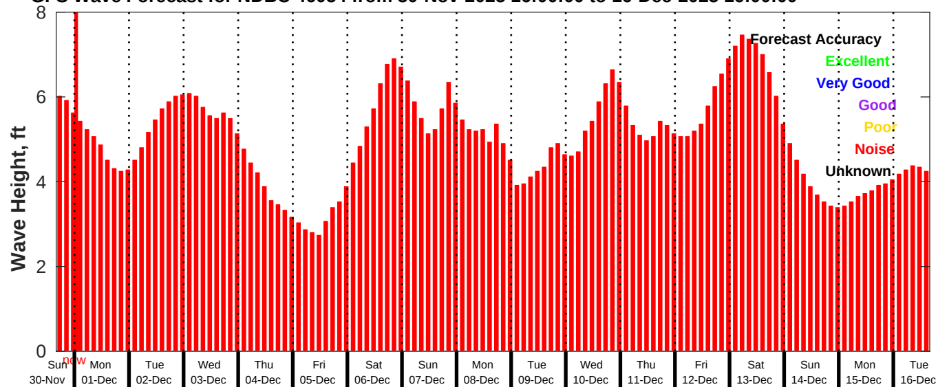
GFS Wave Forecast for NDBC 46054 from 30-Nov-2025 16:00:00 to 16-Dec-2025 16:00:00
