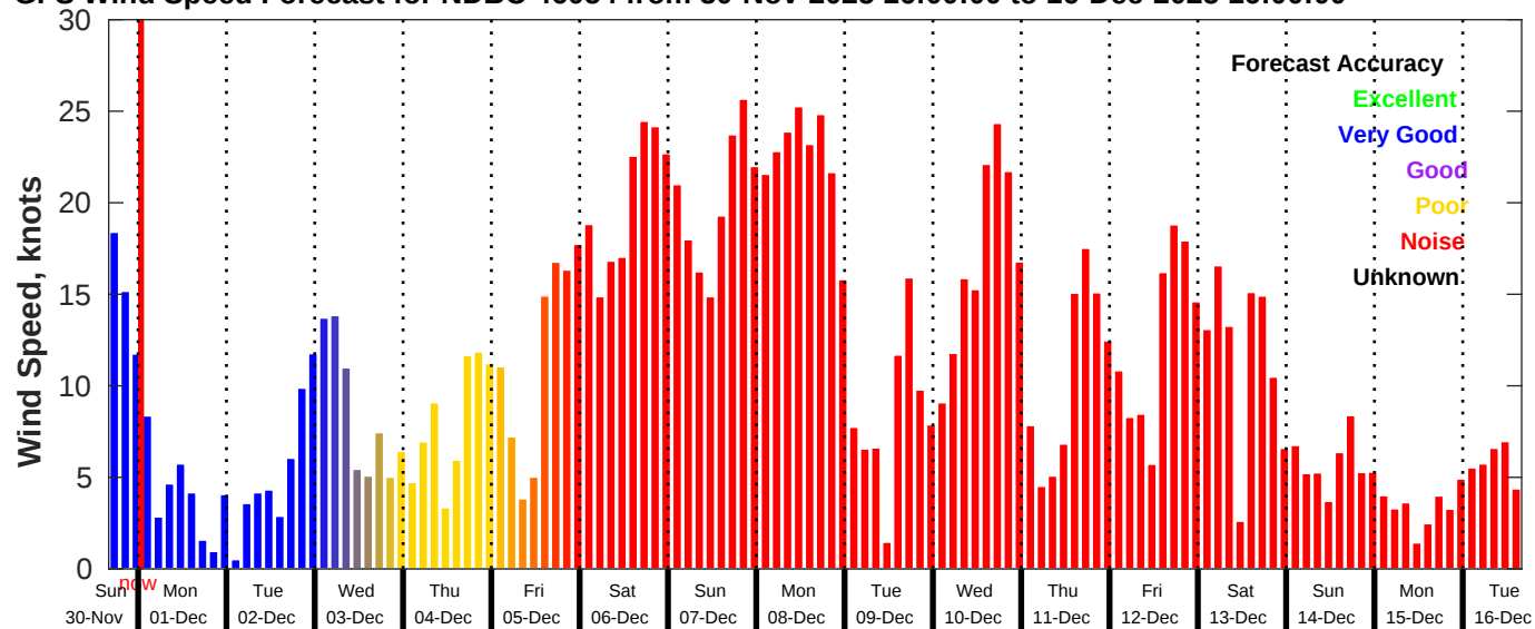
GFS Wind Speed Forecast for NDBC 46054 from 30-Nov-2025 16:00:00 to 16-Dec-2025 16:00:00
