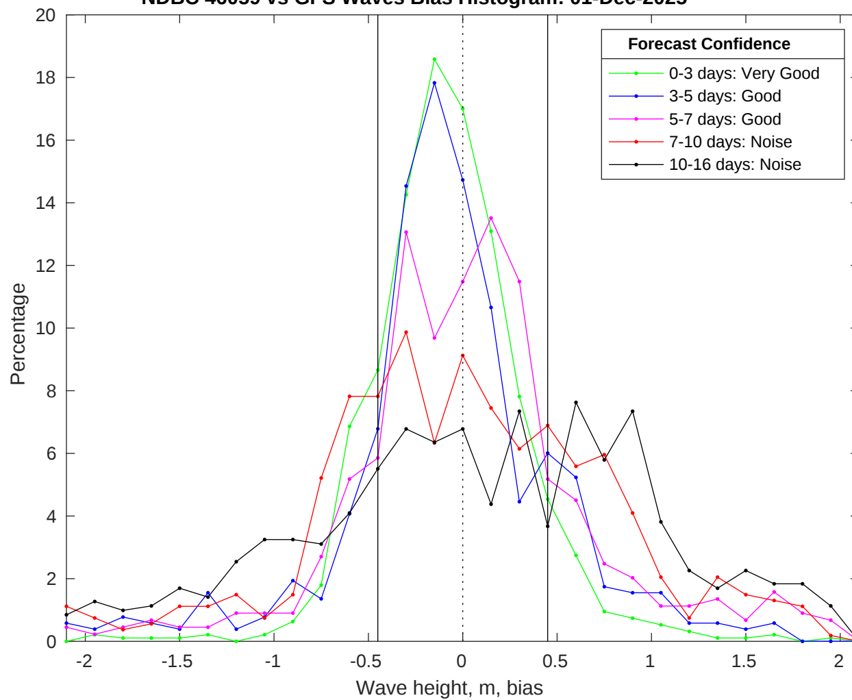
NDBC 46059 vs GFS Waves Bias Histogram: 01-Dec-2025
