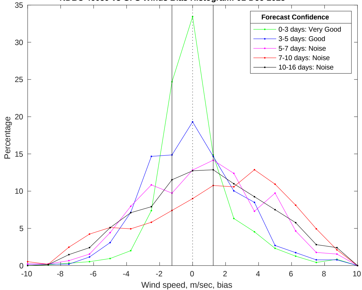
NDBC 46059 vs GFS Winds Bias Histogram: 01-Dec-2025
