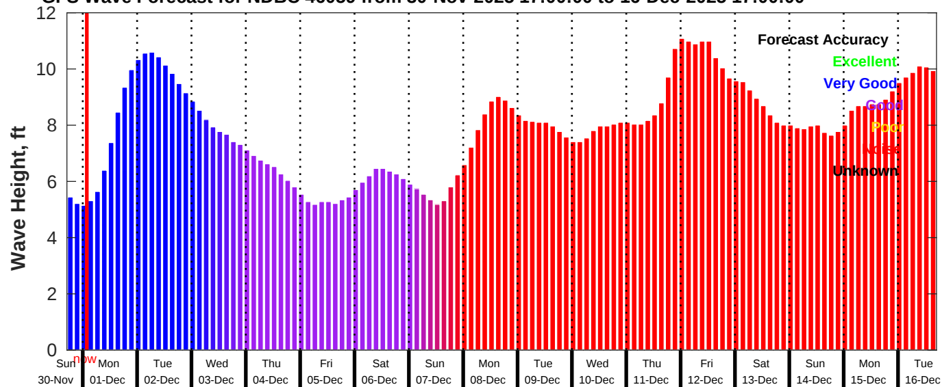
GFS Wave Forecast for NDBC 46059 from 30-Nov-2025 17:00:00 to 16-Dec-2025 17:00:00
