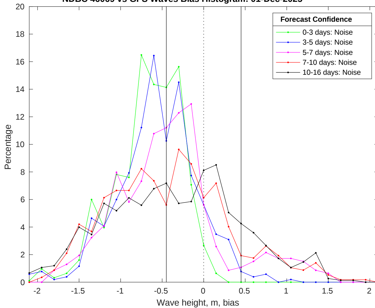
NDBC 46069 vs GFS Waves Bias Histogram: 01-Dec-2025
