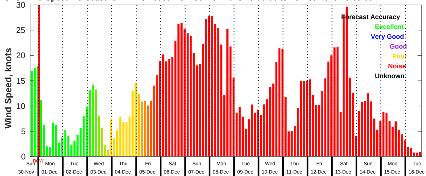
GFS Wind Speed Forecast for NDBC 46069 from 30-Nov-2025 16:00:00 to 16-Dec-2025 16:00:00
