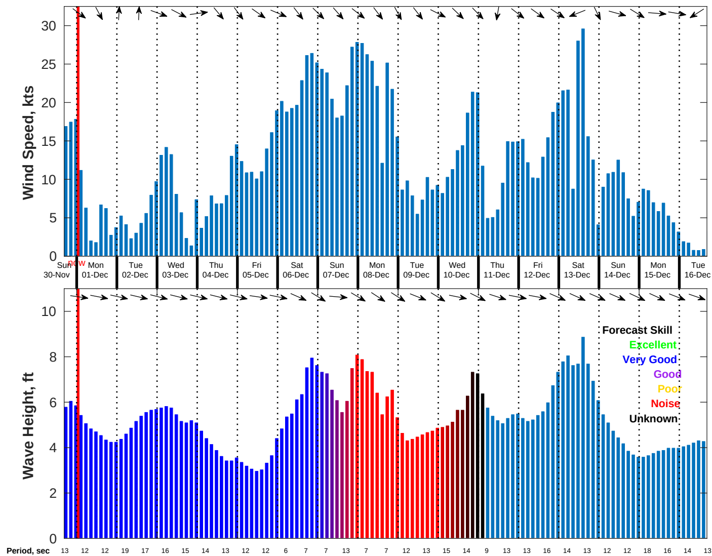
Wind & Wave Forecast for NDBC 46069 from 30-Nov-2025 16:00:00 to 16-Dec-2025 16:00:00
