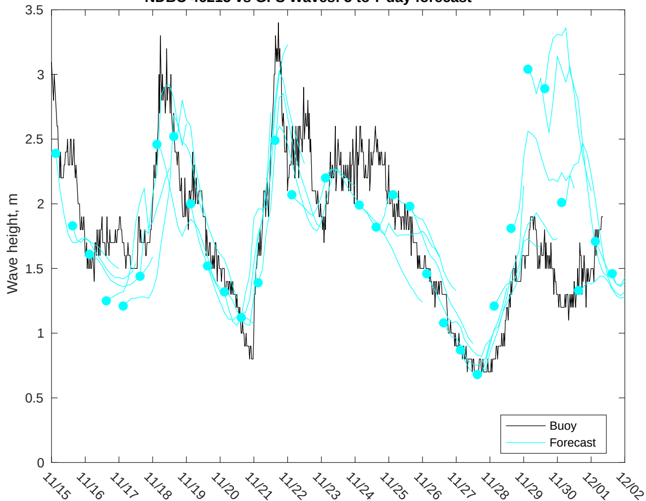
NDBC 46215 vs GFS Waves: 5 to 7 day forecast
