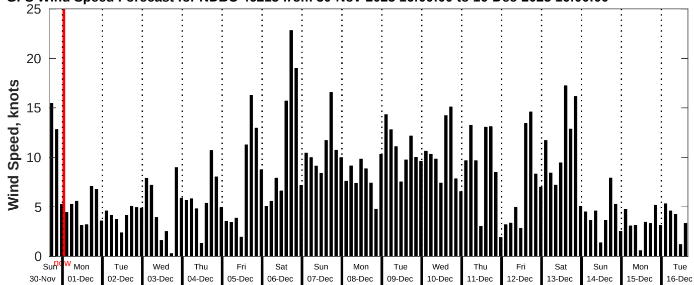
GFS Wind Speed Forecast for NDBC 46215 from 30-Nov-2025 16:00:00 to 16-Dec-2025 16:00:00
