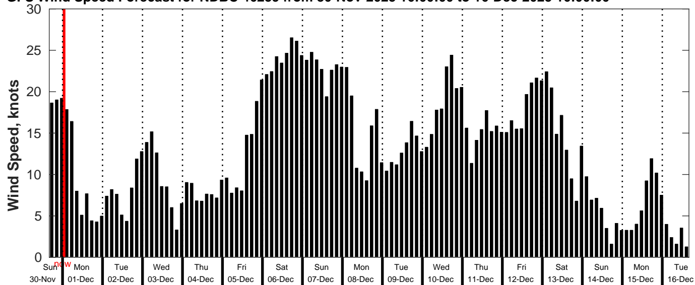
GFS Wind Speed Forecast for NDBC 46259 from 30-Nov-2025 16:00:00 to 16-Dec-2025 16:00:00
