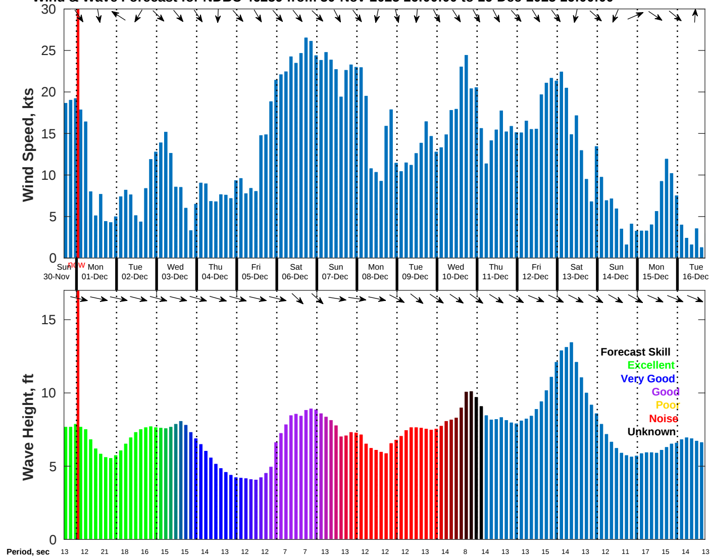
Wind & Wave Forecast for NDBC 46259 from 30-Nov-2025 16:00:00 to 16-Dec-2025 16:00:00
