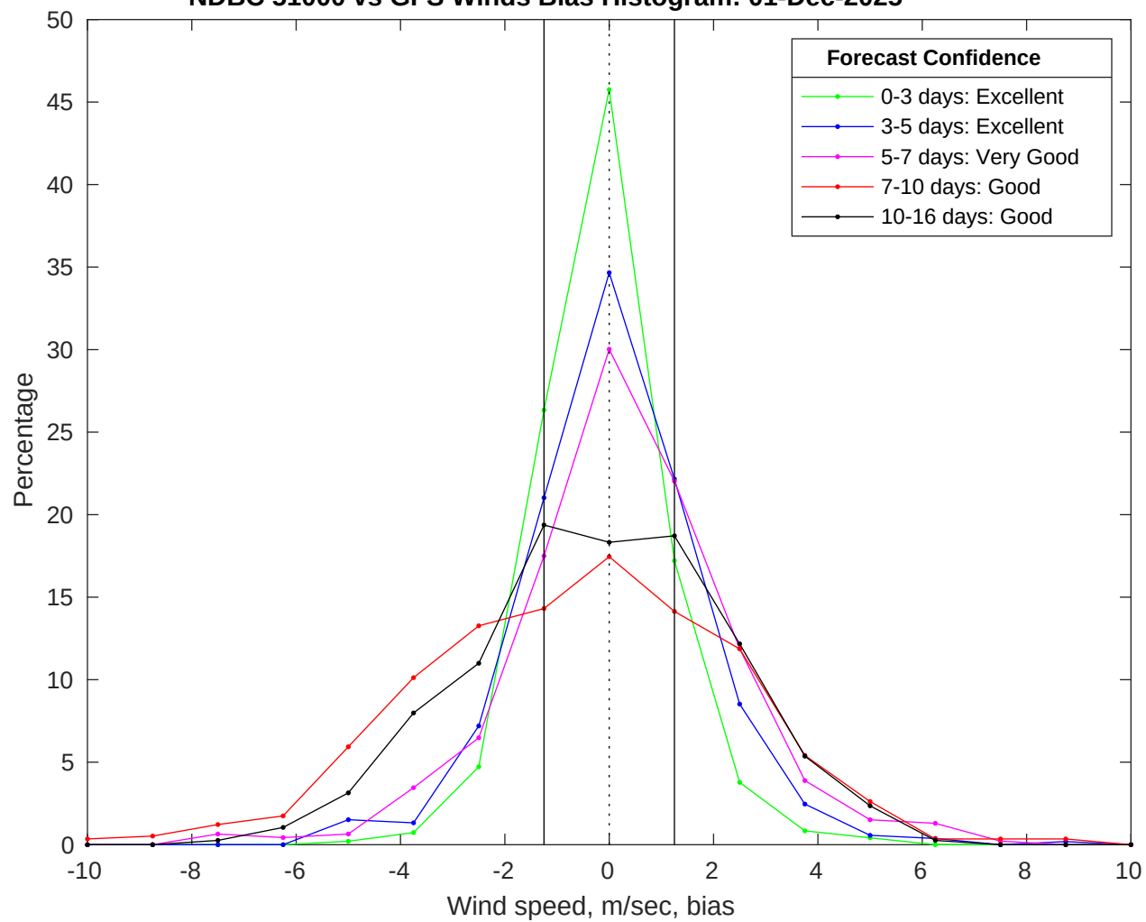
NDBC 51000 vs GFS Winds Bias Histogram: 01-Dec-2025
