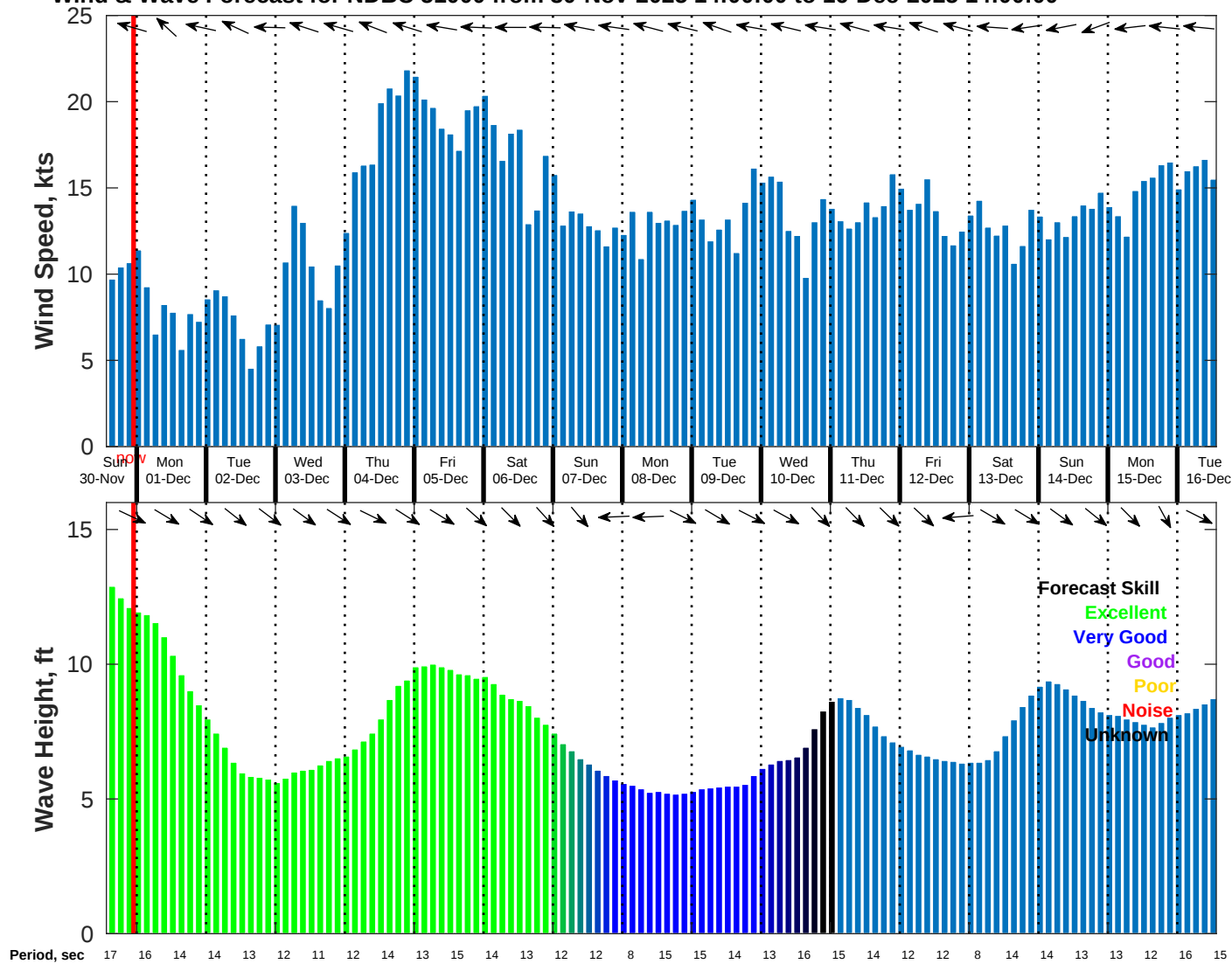
Wind & Wave Forecast for NDBC 51000 from 30-Nov-2025 14:00:00 to 16-Dec-2025 14:00:00
