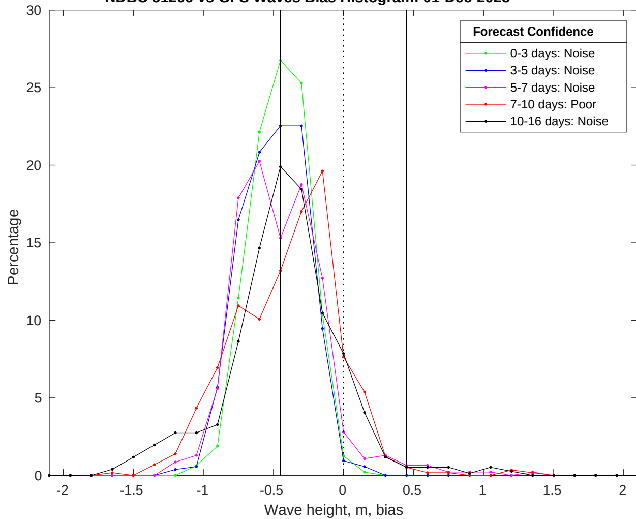
NDBC 51209 vs GFS Waves Bias Histogram: 01-Dec-2025
