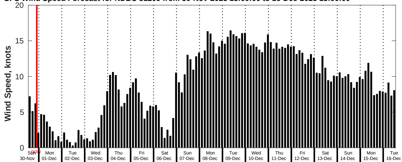
GFS Wind Speed Forecast for NDBC 51209 from 30-Nov-2025 13:00:00 to 16-Dec-2025 13:00:00
