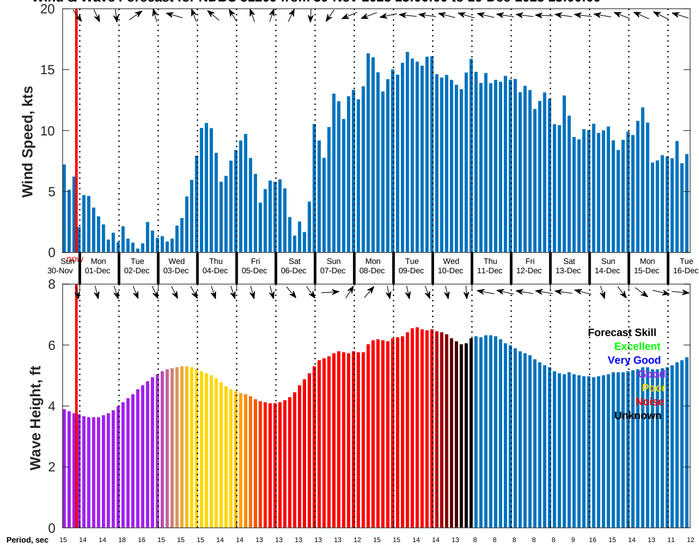
Wind & Wave Forecast for NDBC 51209 from 30-Nov-2025 13:00:00 to 16-Dec-2025 13:00:00
