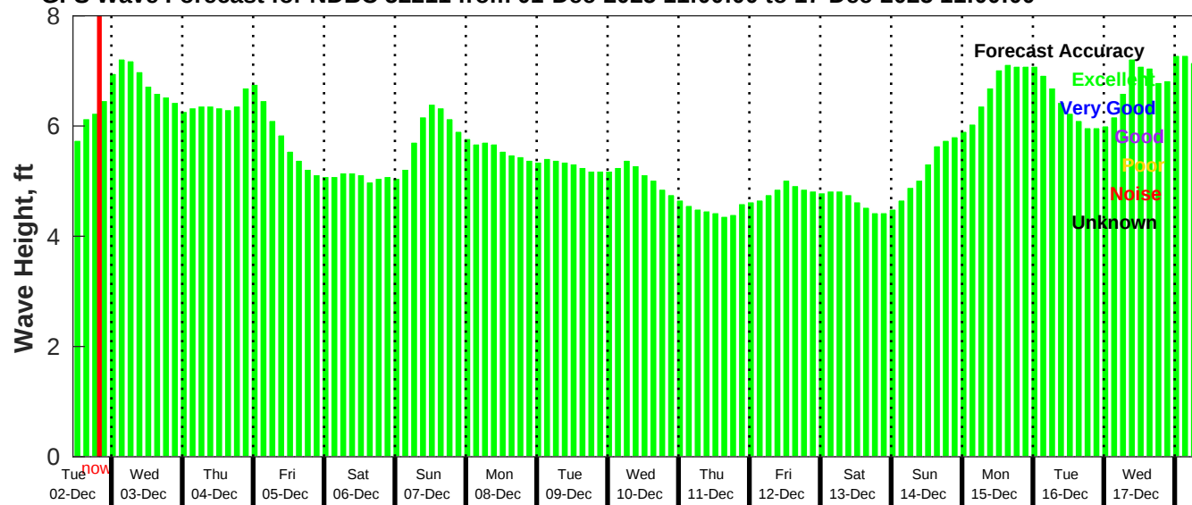
GFS Wave Forecast for NDBC 52211 from 01-Dec-2025 11:00:00 to 17-Dec-2025 11:00:00
