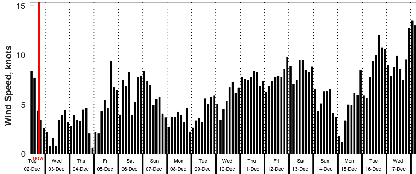
GFS Wind Speed Forecast for NDBC 52212 from 01-Dec-2025 09:00:00 to 17-Dec-2025 09:00:00
