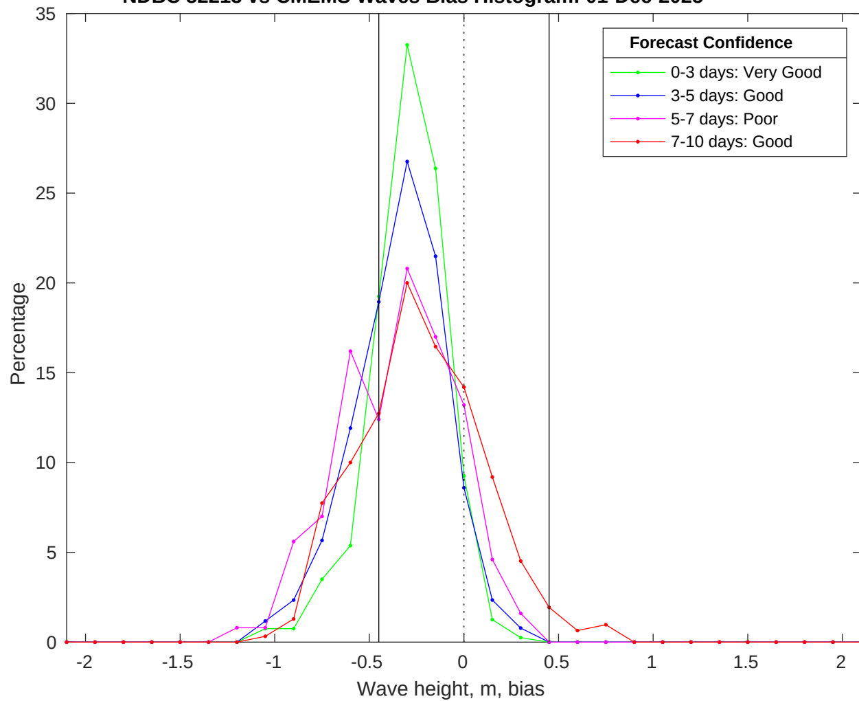
NDBC 52213 vs CMEMS Waves Bias Histogram: 01-Dec-2025
