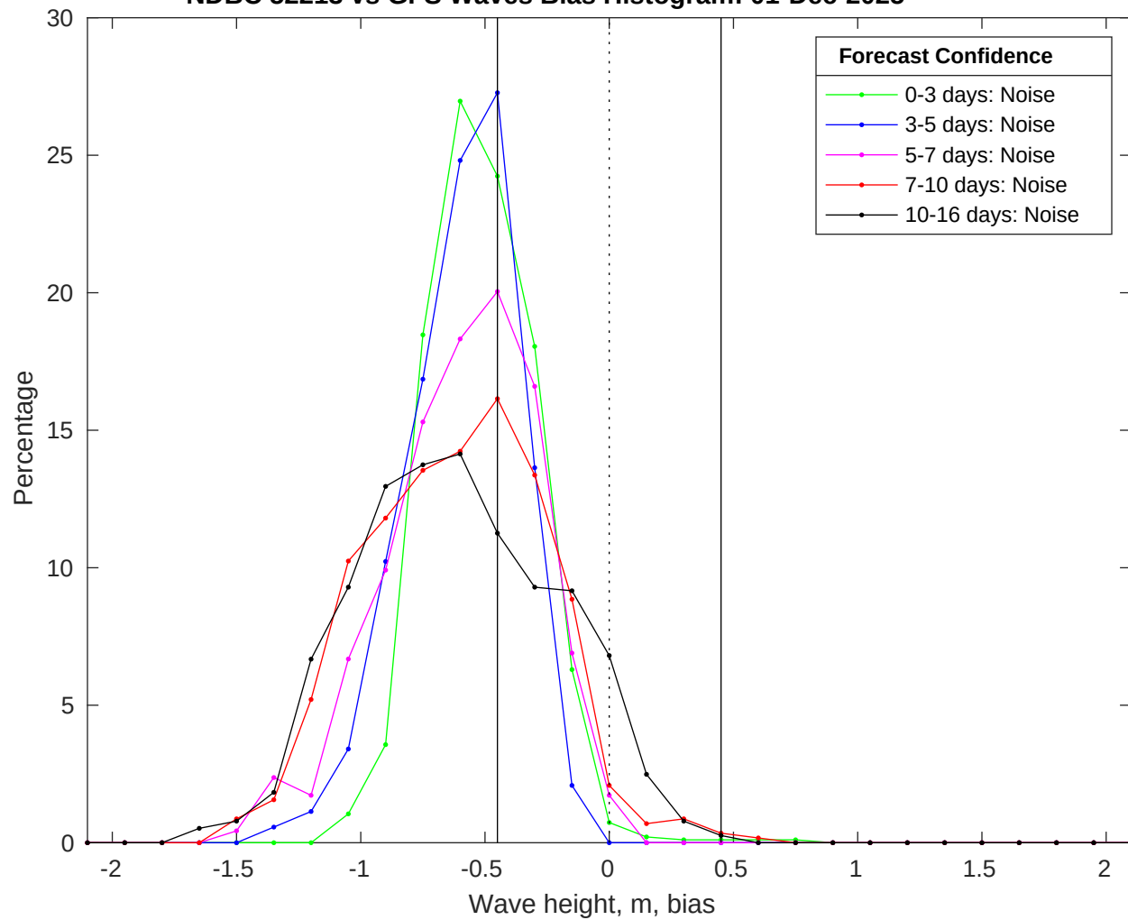
NDBC 52213 vs GFS Waves Bias Histogram: 01-Dec-2025
