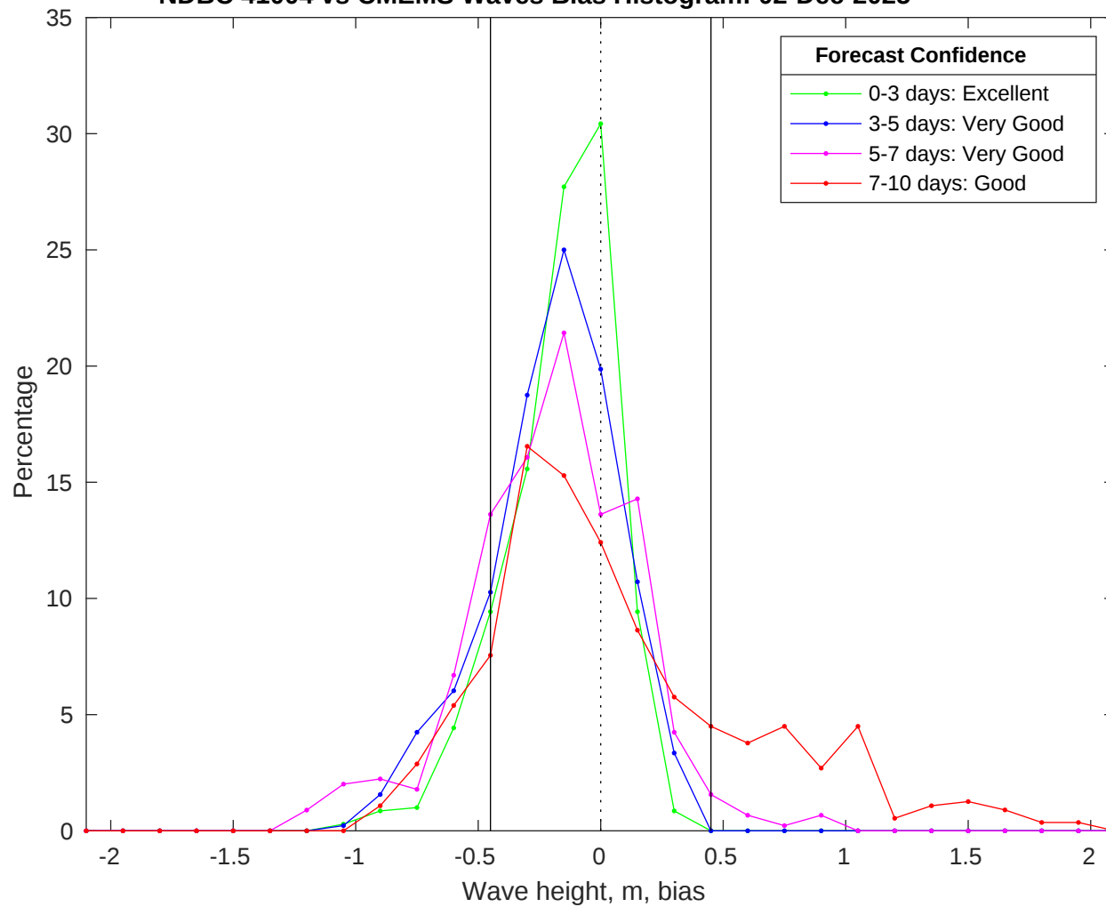
NDBC 41004 vs CMEMS Waves Bias Histogram: 02-Dec-2025
