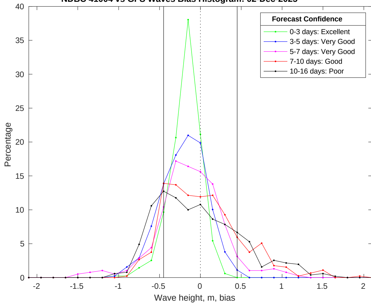
NDBC 41004 vs GFS Waves Bias Histogram: 02-Dec-2025
