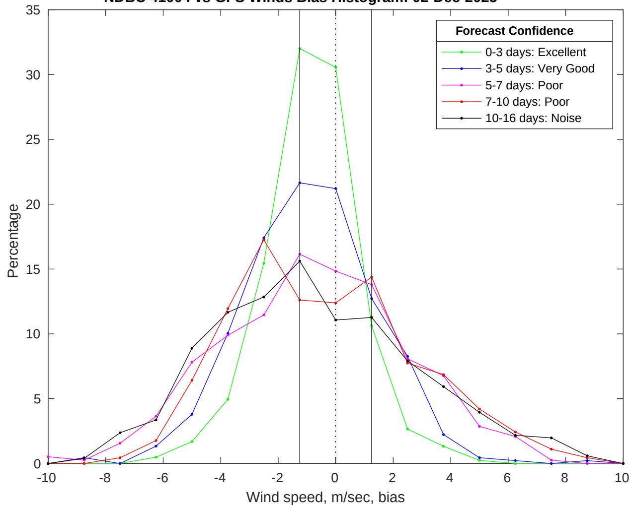
NDBC 41004 vs GFS Winds Bias Histogram: 02-Dec-2025
