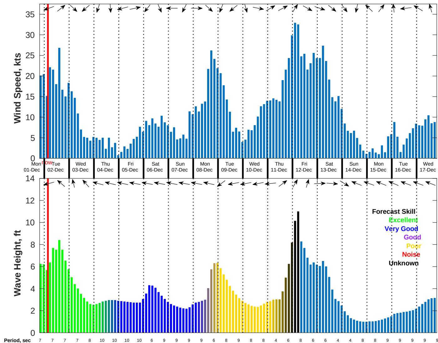
Wind & Wave Forecast for NDBC 41004 from 01-Dec-2025 19:00:00 to 17-Dec-2025 19:00:00
