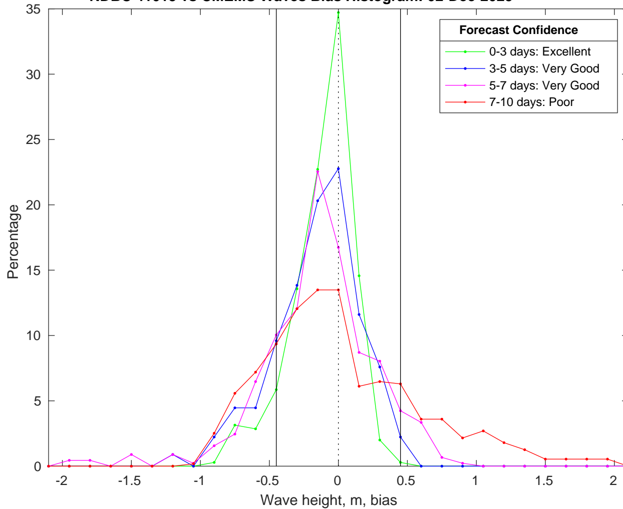
NDBC 41013 vs CMEMS Waves Bias Histogram: 02-Dec-2025
