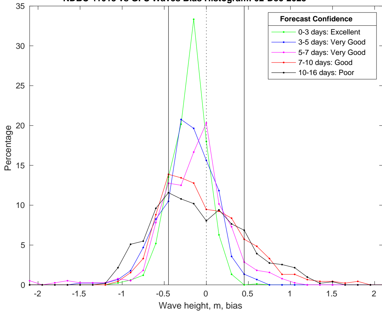
NDBC 41013 vs GFS Waves Bias Histogram: 02-Dec-2025
