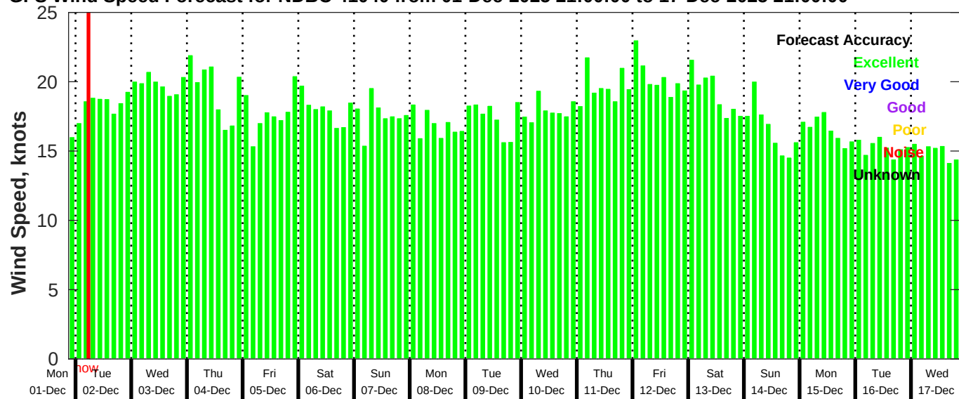
GFS Wind Speed Forecast for NDBC 41040 from 01-Dec-2025 21:00:00 to 17-Dec-2025 21:00:00
